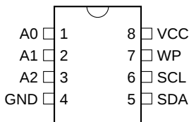
8-ball dBG2
