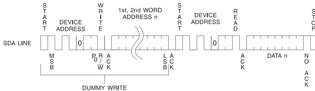
Figure 12. Sequential Read
