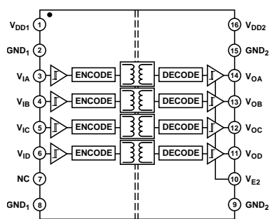
Figure 1. ADuM1400 Functional Block Diagram
