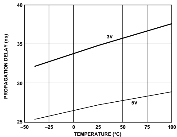
Figure 16. Propagation Delay vs. Temperature, C Grade
