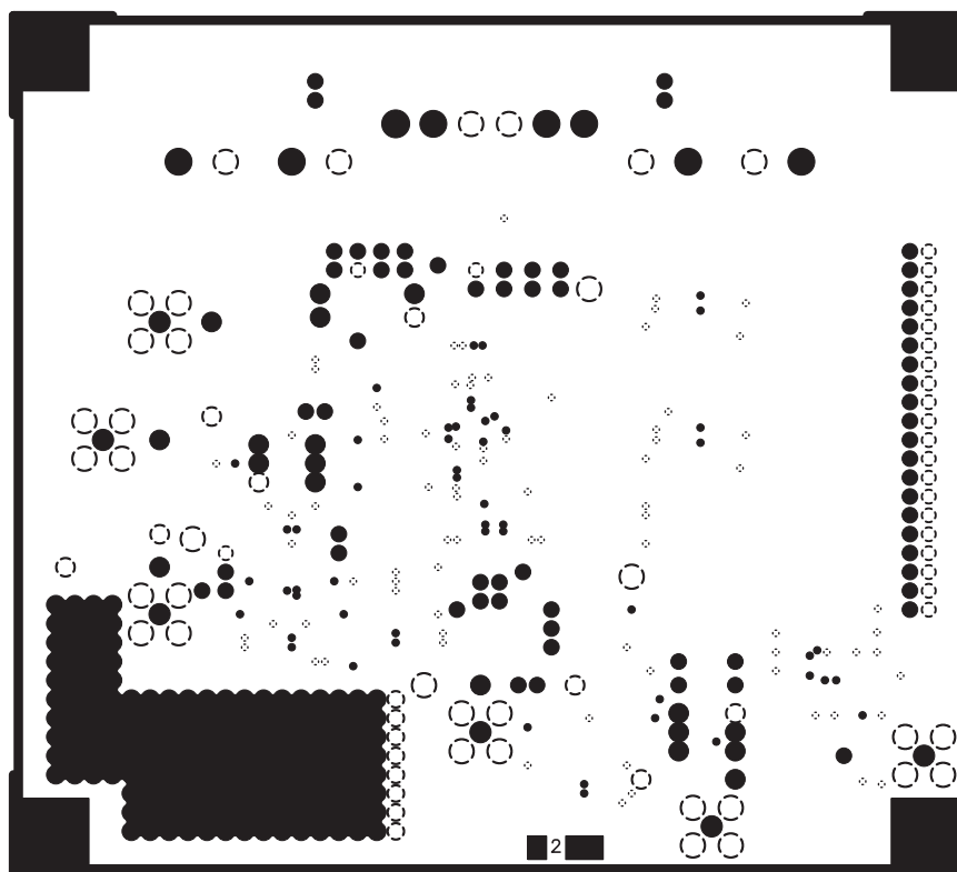
Figure 23. TSSOP Evaluation Board Layout, Ground Plane
