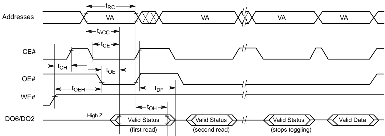
Figure 12. Data# Polling Timings (During Embedded Algorithms)
