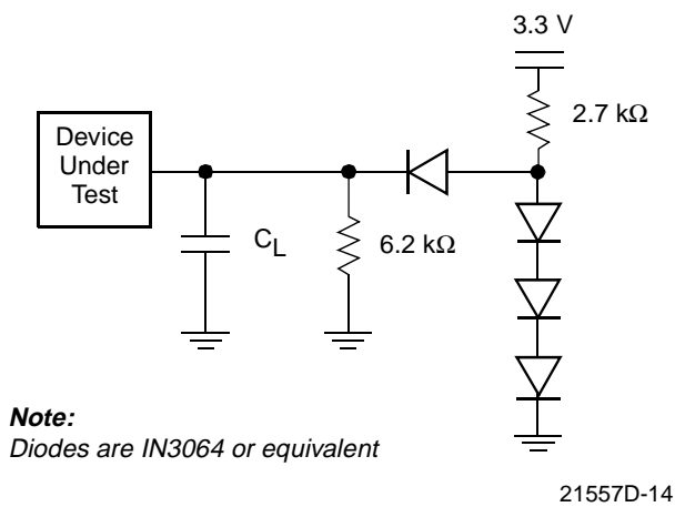
Figure 6. Test Setup
