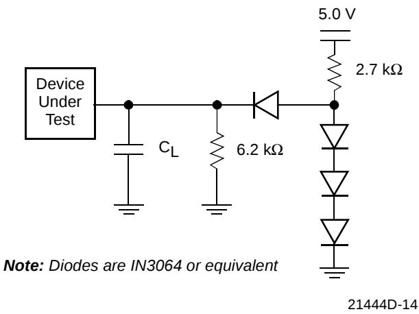
Figure 8. Test Setup
