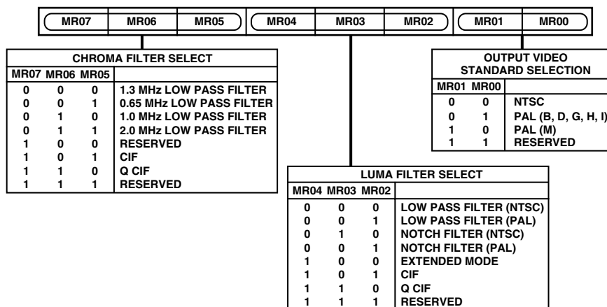
Figure 38. Mode Register 0
