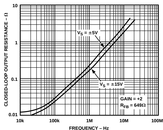
Figure 8. Closed-Loop Output Resistance vs. Frequency
