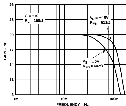
Figure 23. Closed-Loop Gain vs. Frequency, Gain = +10
