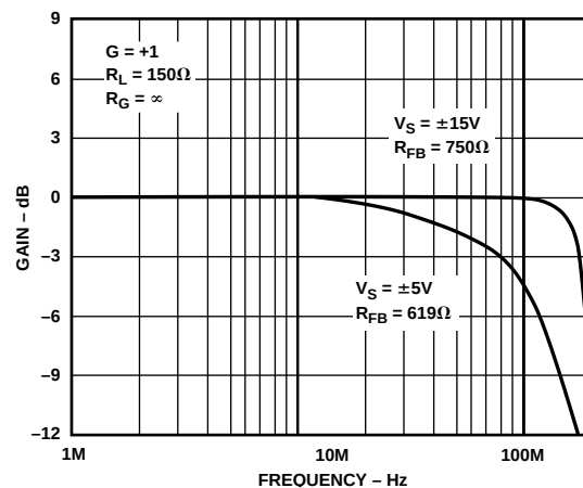
Figure 22. Closed-Loop Gain vs. Frequency, Gain = +1
