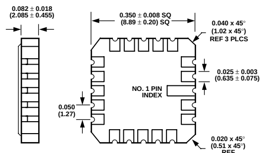
20-Lead LCC (E-20A) Package
