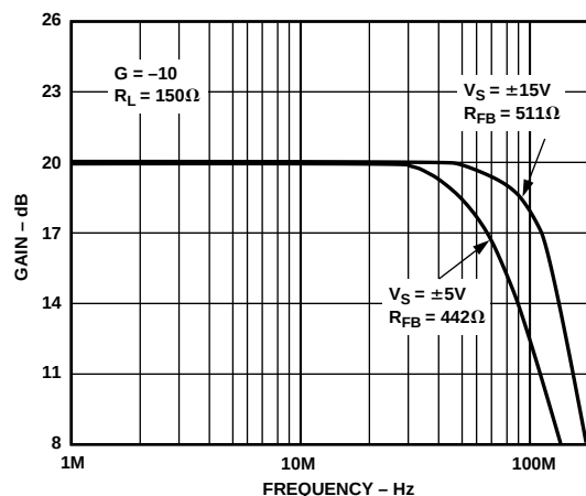
Figure 29. Closed-Loop Gain vs. Frequency, Gain = -10
