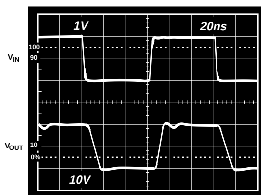
Figure 24. Large Signal Pulse Response, Gain = +10
