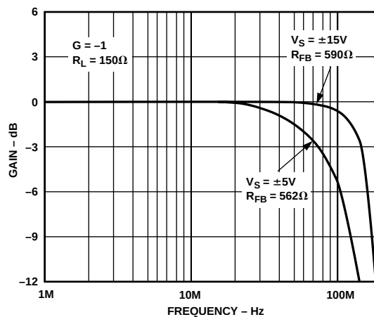
Figure 28. Closed-Loop Gain vs. Frequency, Gain = -1
