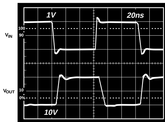
Figure 30. Large Signal Pulse Response, Gain = -10
