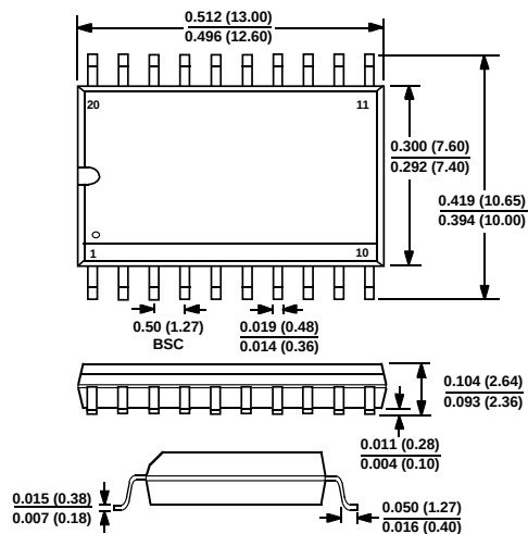
20-Lead Wide Body SOIC (R-20) Package
