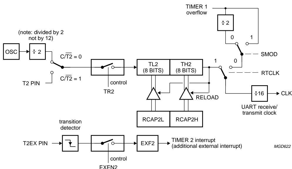
Fig.18 Timer 2 in Baud Rate Generator mode.
