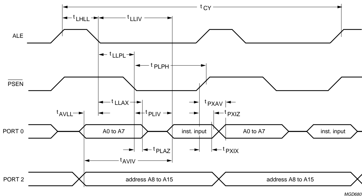
Fig.41 Read from Program Memory.
