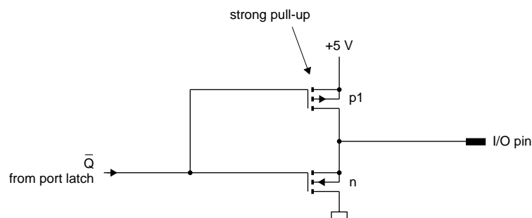
(c) Push-pull
