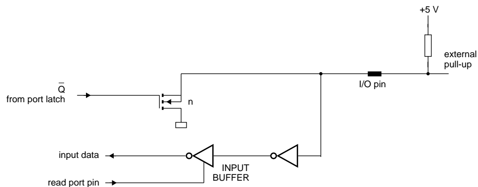
(b) Open-drain
