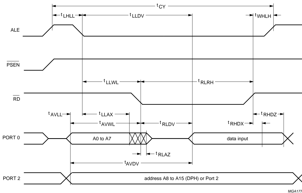
Fig.42 Read from Data Memory.
