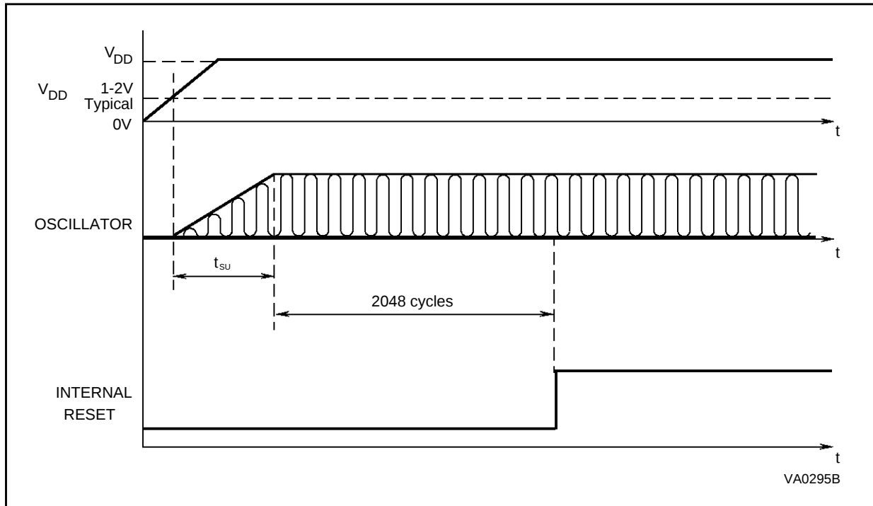
Figure 33. Power-on-Reset
