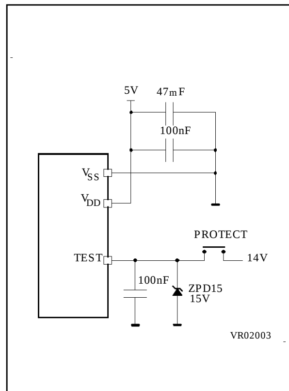
Figure 40. Programming Circuit
