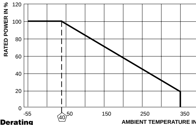
Derating
