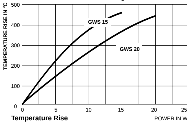
Temperature Rise
