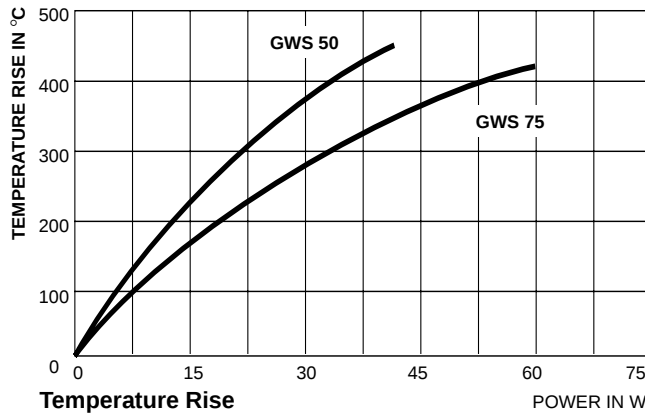
Temperature Rise
