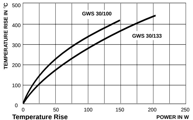
Temperature Rise
