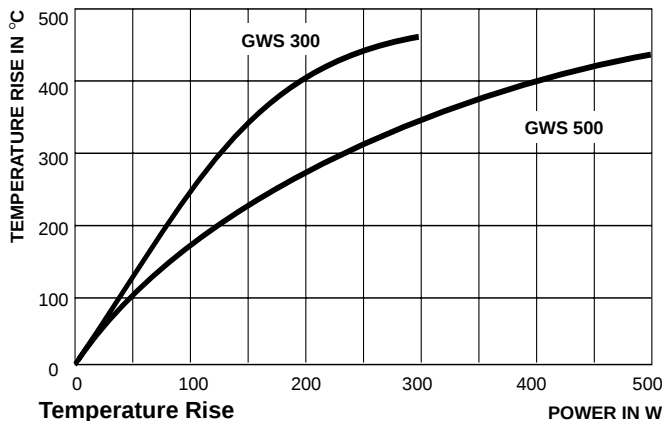
Temperature Rise
