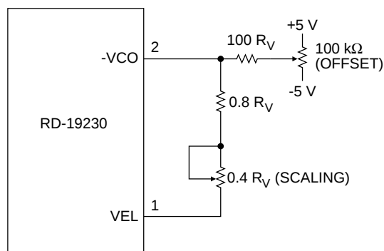
FIGURE 15. VELOCITY TRIMMING
