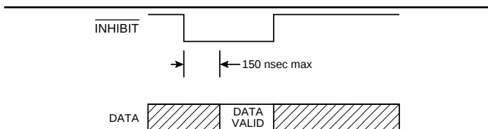
FIGURE 18. INHIBIT TIMING
