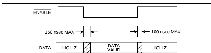
FIGURE 19. ENABLE TIMING
