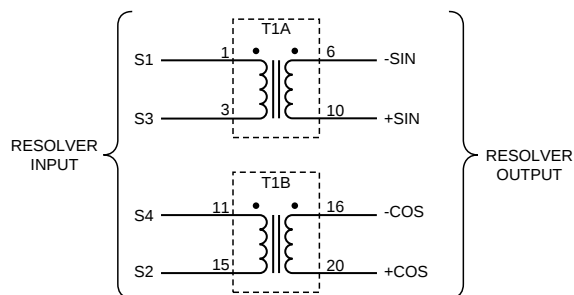
FIGURE 7. TRANSFORMER LAYOUT AND SCHEMATIC (RESOLVER INPUT - 52036/52037/52038)
