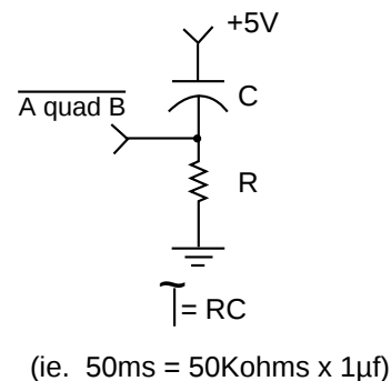
FIGURE 23B. EXAMPLE RESET CIRCUIT FOR A QUAD B RESET
