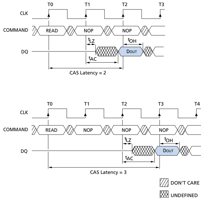
Figure 2 CAS Latency
