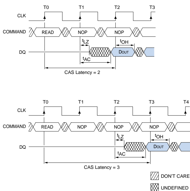
Figure 6 CAS Latency
